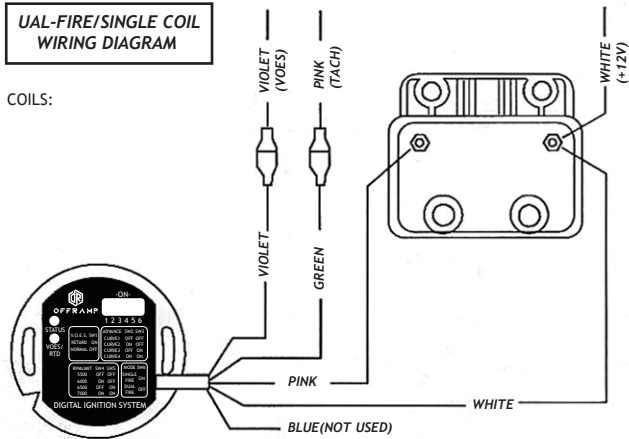
SINGLE-FIRE/SINGLE COIL WIRING DIAGRAM
